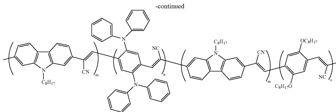
PCVDPAP (Knoevenagel Reaction)
