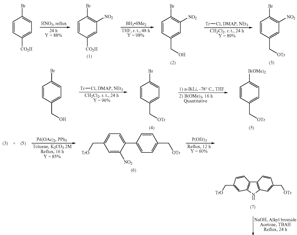
Scheme 1: Synthetic Route to 2,7-difunctionalized carbazole
