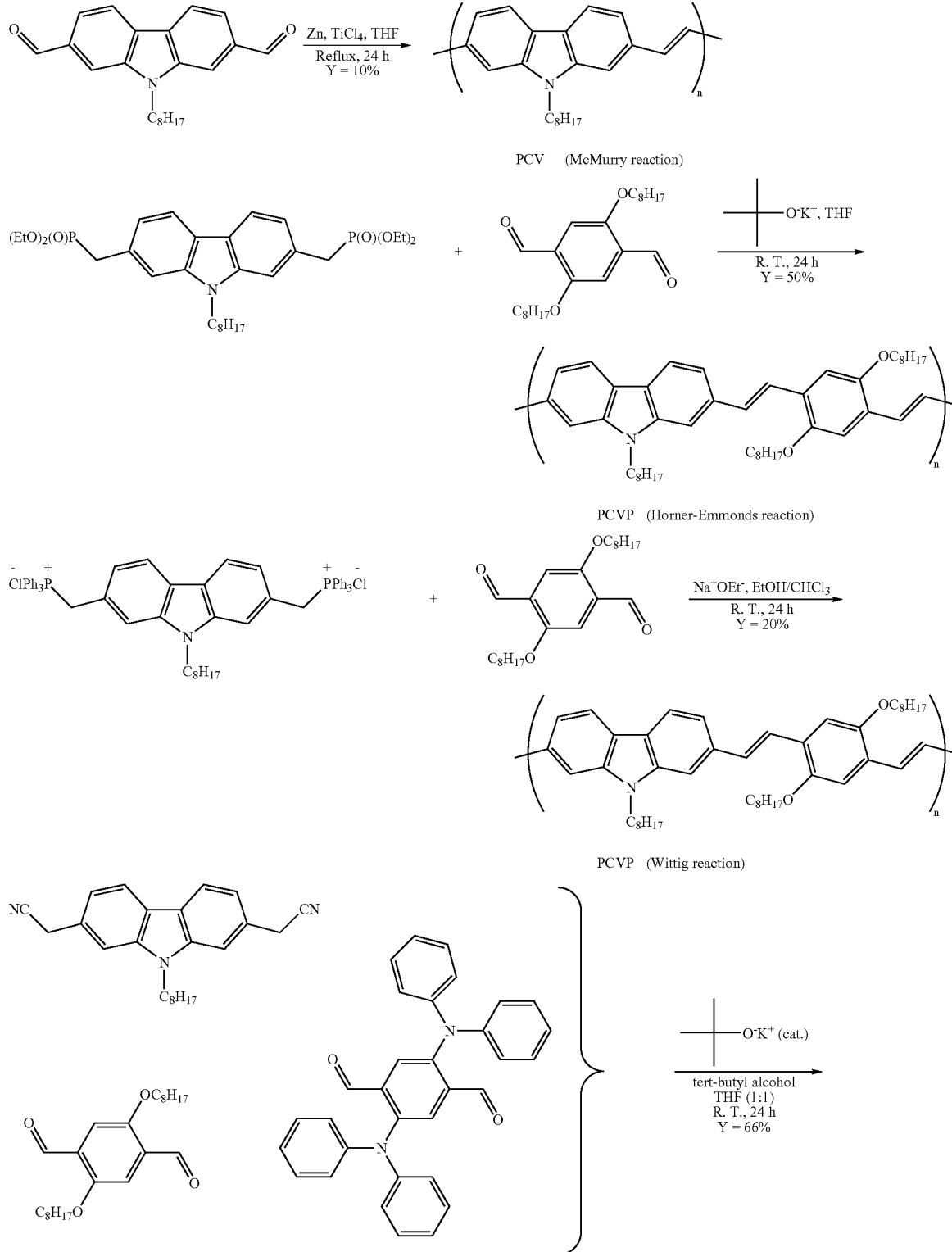
Scheme 4: Synthetic Route to 2,7-carbazolenevinylene polymers
