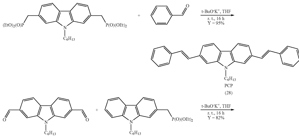
Scheme 3: Synthetic Route to 2,7-carbazolenevinylene oligomers
